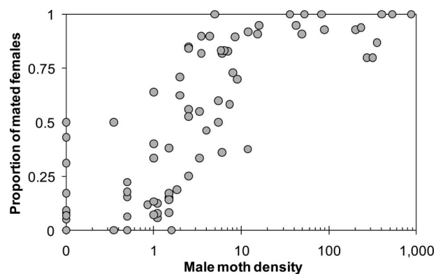
Figure 3. Results of field studies showing that the mating success of L. dispar females is influenced by the background male moth density (Sharov et al. 1995; Tcheslavskaja et al. 2002; Contarini et al. 2009).
