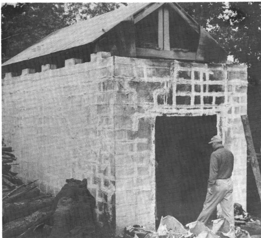
The cinder-block kiln is well suited for small charcoal operations. This kiln has a capacity of 9 cords.
